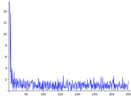
FIGURE 7. Minimum moduli for h_n = \lambda_n before deformation.
